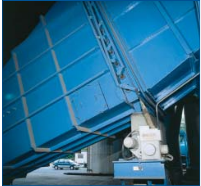
Beck drive installed on a parallel blade inlet damper.
