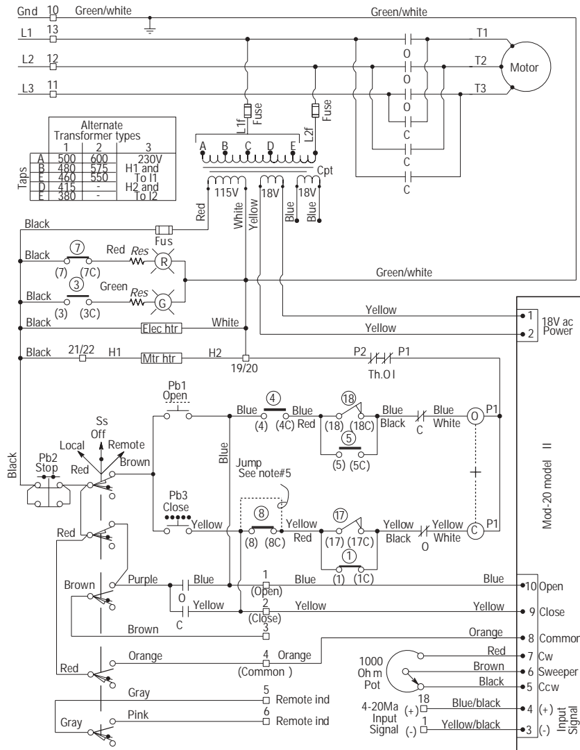
Figure 8.1 – Modutronic 20 II Typical 3-Phase Wiring Diagram
