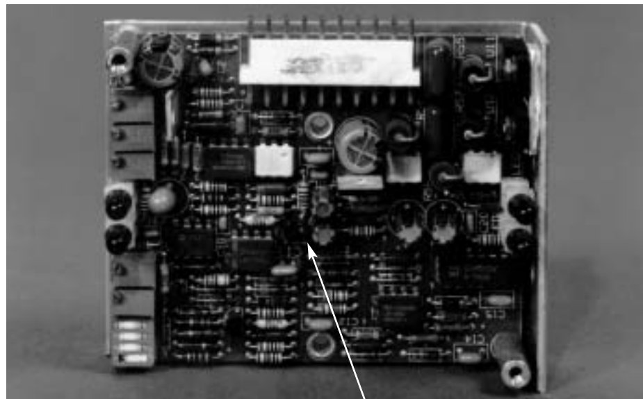
Figure 6.4 – FAIL TO Mode JP1 Jumper
