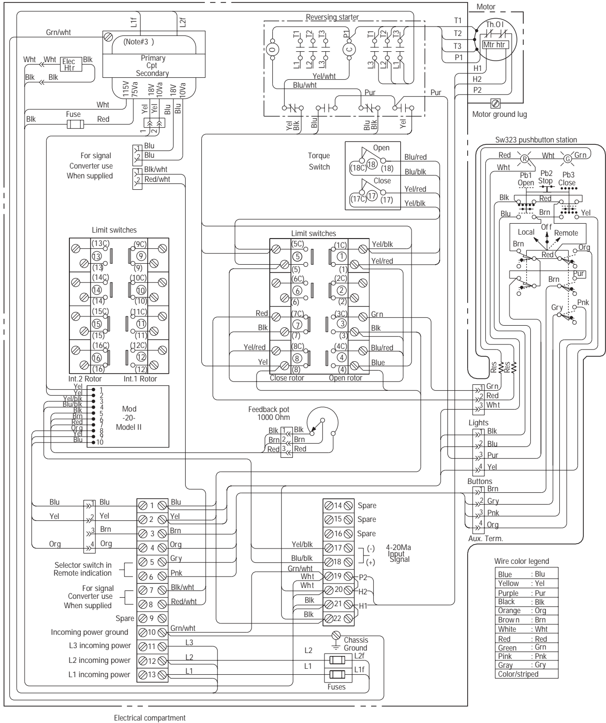
Figure 8.1 – Modutronic 20 II Typical 3-Phase Wiring Diagram (continued)
