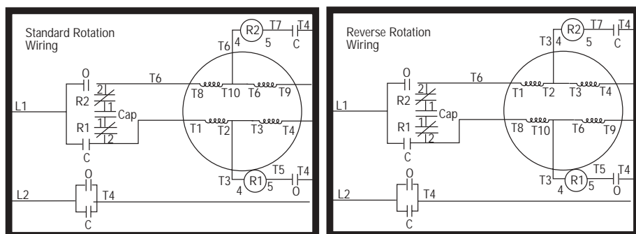
Figure 4.2 – Standard Motor Rotation & Reverse Motor Rotation Wiring Diagrams for Dual Voltage, Capacitor Start, Induction Run, and Single-Phase High-Voltage Motors
