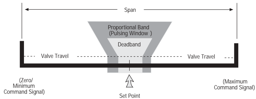
Figure 3.1 – Calibration Positions
