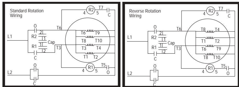
Figure 4.1 – Standard Motor Rotation & Reverse Motor Rotation Wiring Diagrams for Dual Voltage, Capacitor Start, Induction Run, and Single-Phase Low-Voltage Motors
