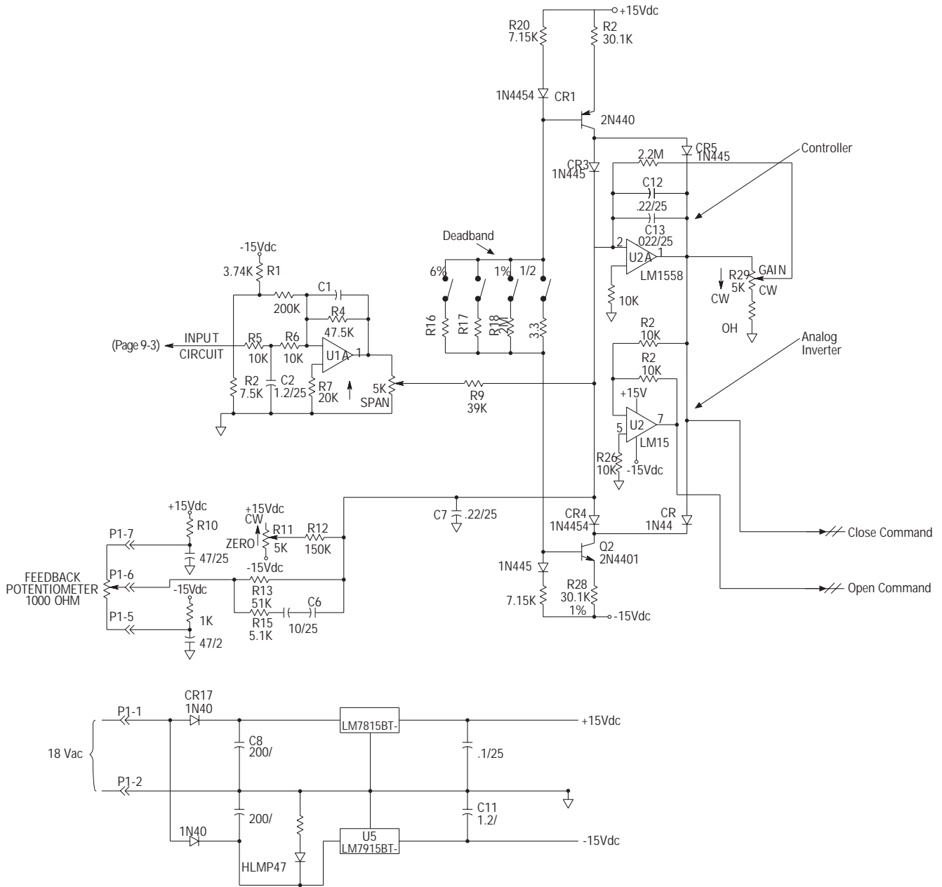
Figure 9.1 – Modutronic 20 II Schematic Diagram
