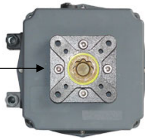
Models: J3-55 and J3-85 Mounting: F05, and F07 50mm and 70mm PCD Output: 17mm double square (star) 14mm option
